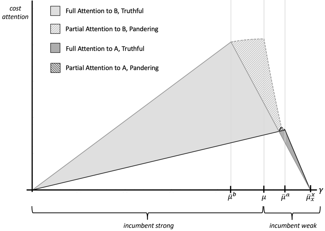
Figure 4: Asymmetric attention equilibria with moderate information
